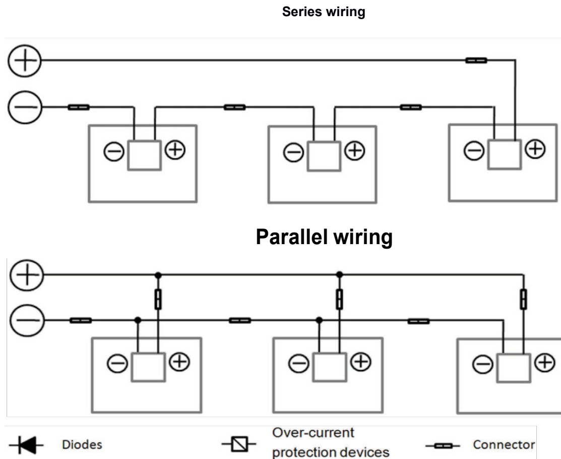
Figure 1: Electrical diagrams of series and parallel wiring.
